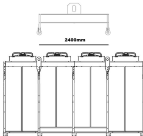
SJ 2x4 - Total 4 lifting points
