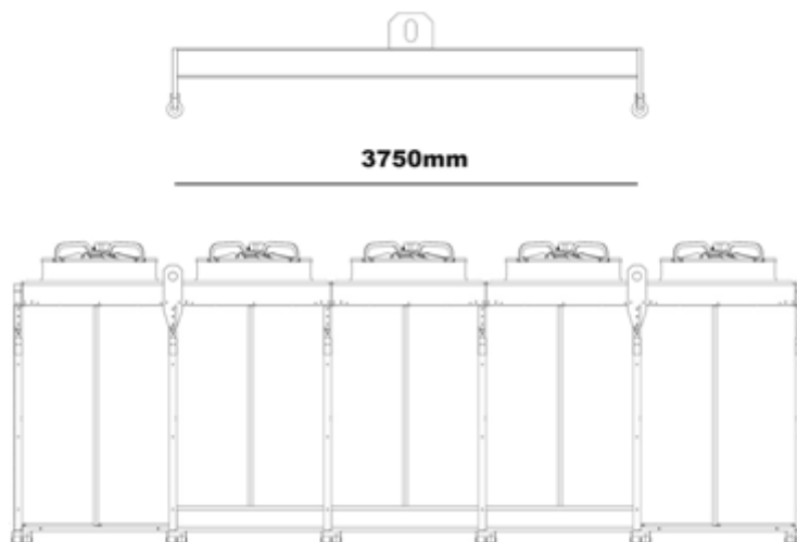
JV 2x5 - Total 4 lifting points
