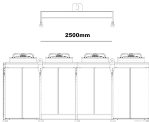
JV 2x4 - Total 4 lifting points
